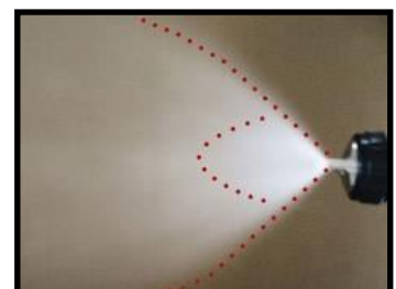
Closing Pattern of a Dirty Spray Gun
